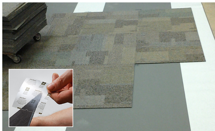
GroundBridge strips (shown in white). Inset: TacTiles square being applied to corner of carpet tile.
