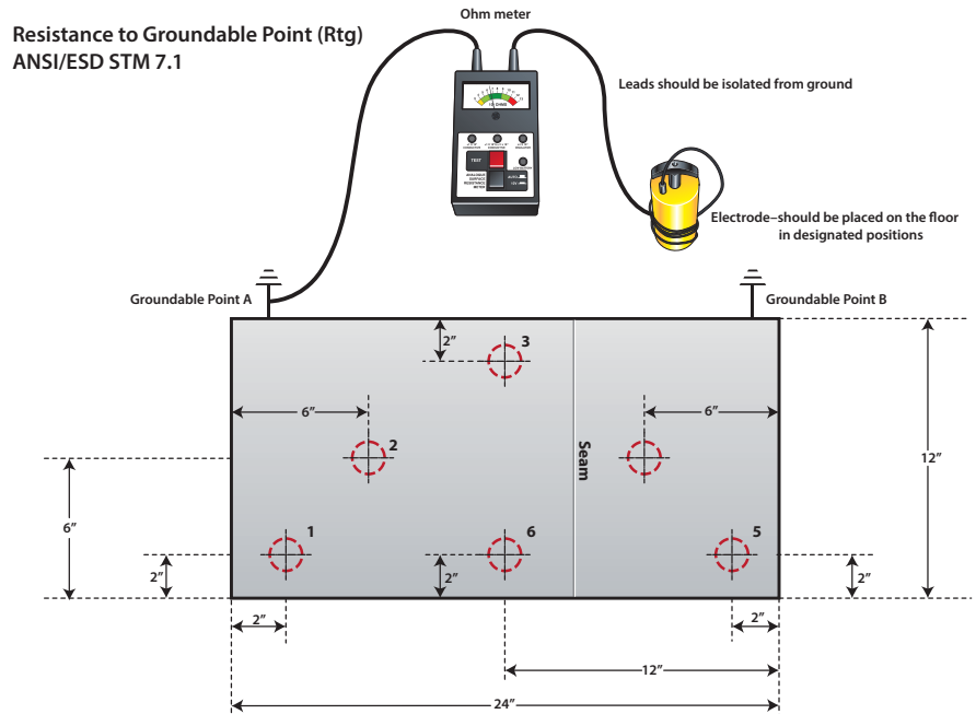
Figure 3: Using the test leads and one 5 pound electrode to measure RTG
