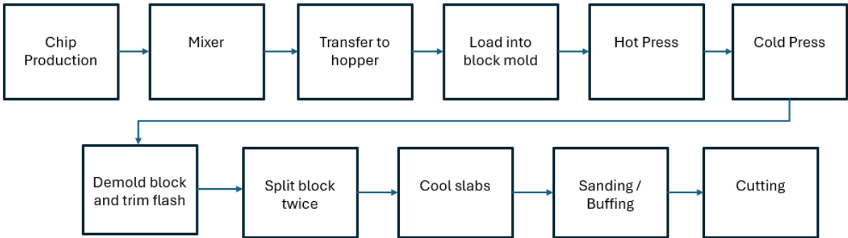
Flow Diagram
